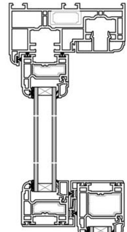
VERTICAL SECTION WITH DEEP BOTTOM RAIL
