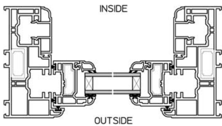
HORIZONTAL SECTION THROUGH TOP SASH
