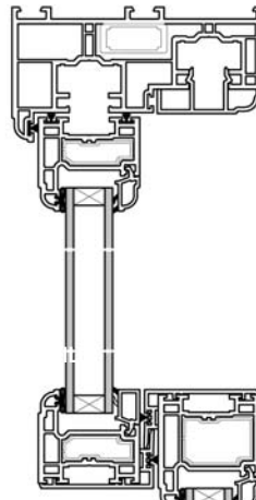
VERTICAL SECTION WITH STANDARD BOTTOM RAIL
