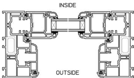
HORIZONTAL SECTION THROUGH BOTTOM SASH
