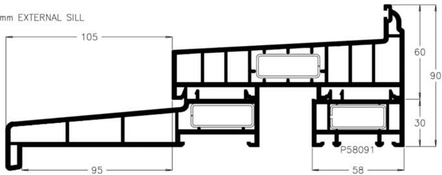
P01044 200mm EXTERNAL SILL
